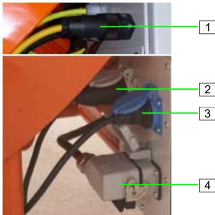
Abb. 35: Stromanschlüsse
