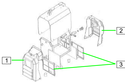
Abb. 92: Filter reinigen
